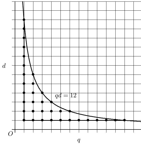
FIGURE 1. Dirichlet's divisor problem
